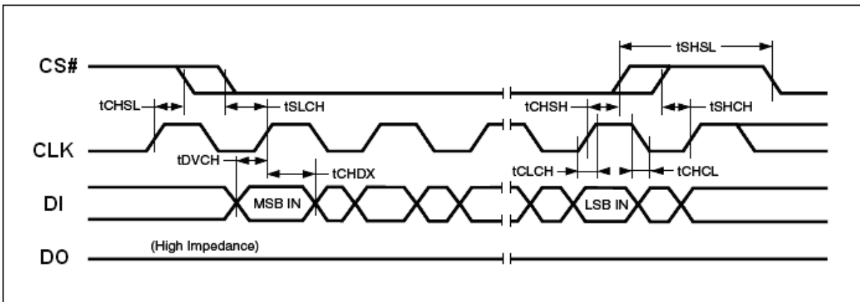
Figure 33. Input Timing
