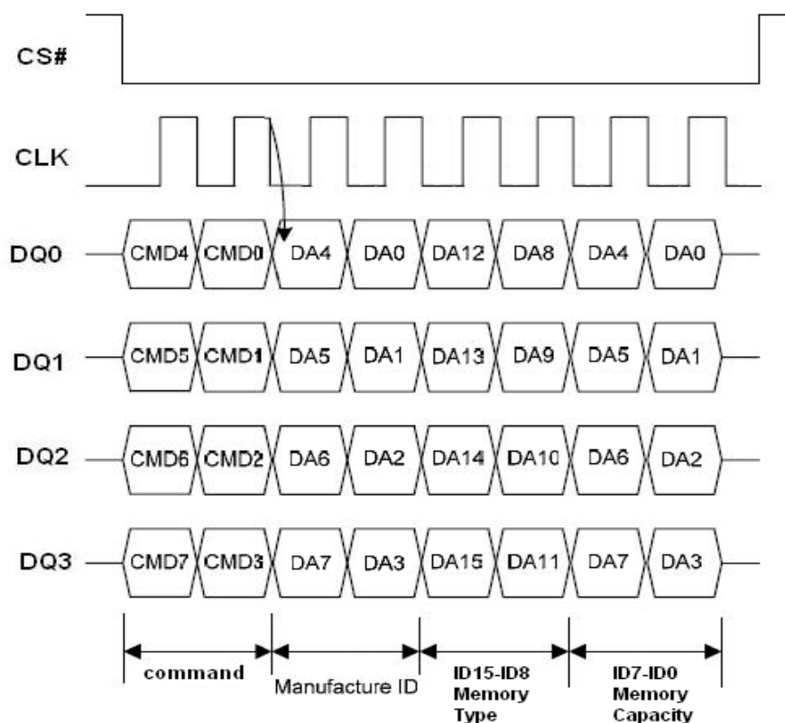
Figure 27.1. Read Identification (RDID) in QPI Mode
