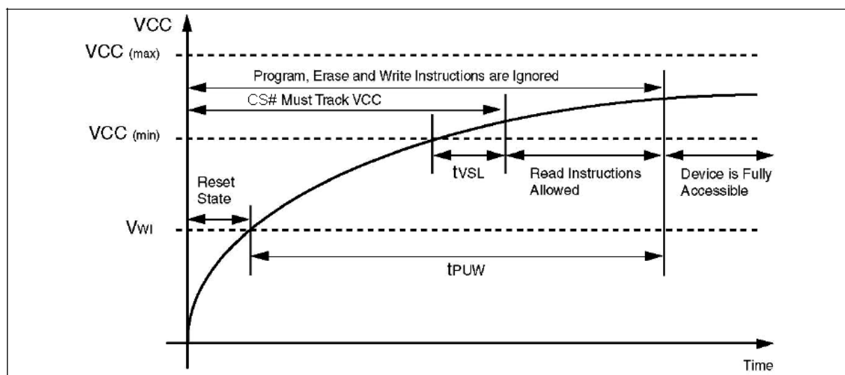
Figure 30. Power-up Timing
