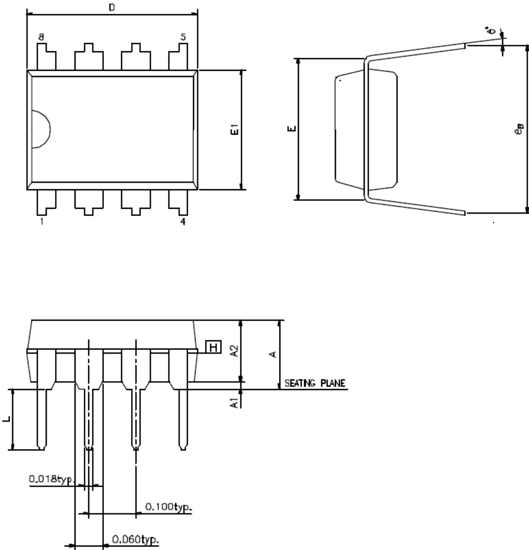
Figure 39. PDIP8
