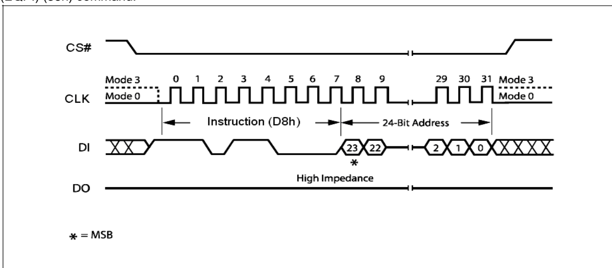
Figure 21. 64KB Block Erase Instruction Sequence Diagram
