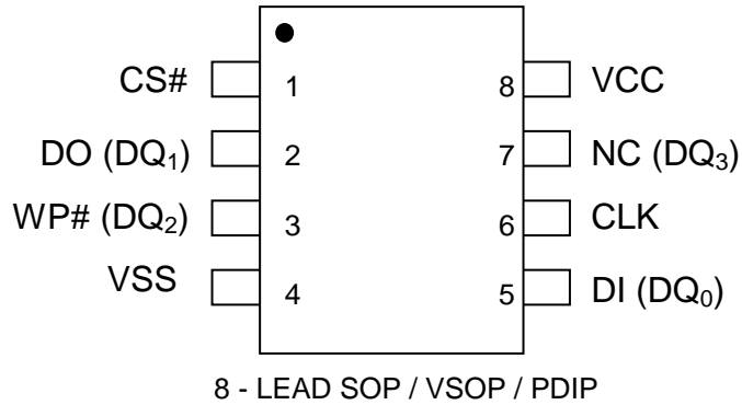
Figure.1 CONNECTION DIAGRAMS
