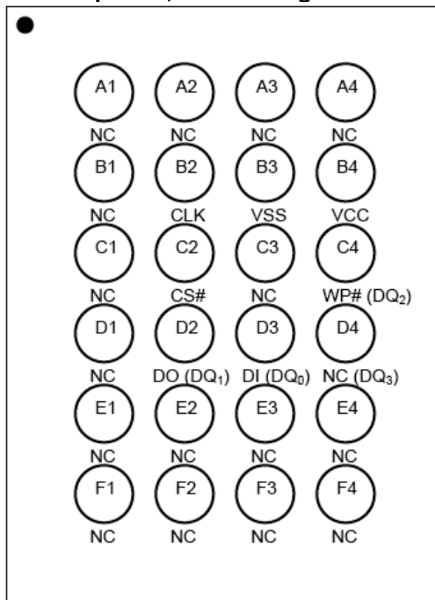
24 - Ball TFBGA
