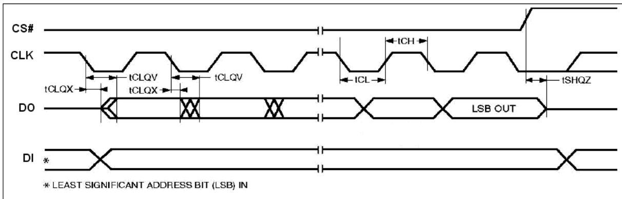
Figure 32. Serial Output Timing
