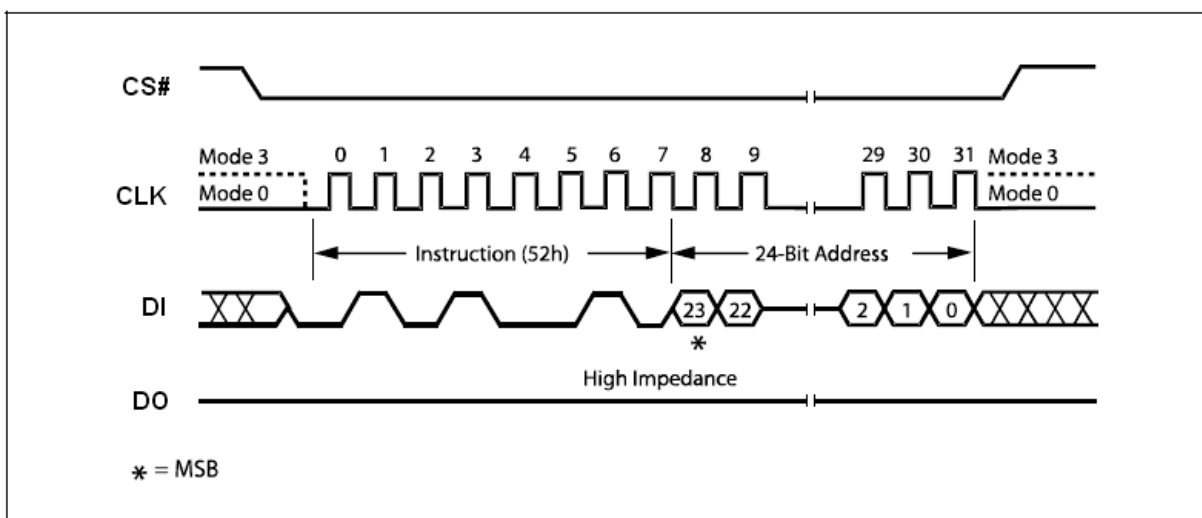
Figure 20. 32KB Half Block Erase Instruction Sequence Diagram
