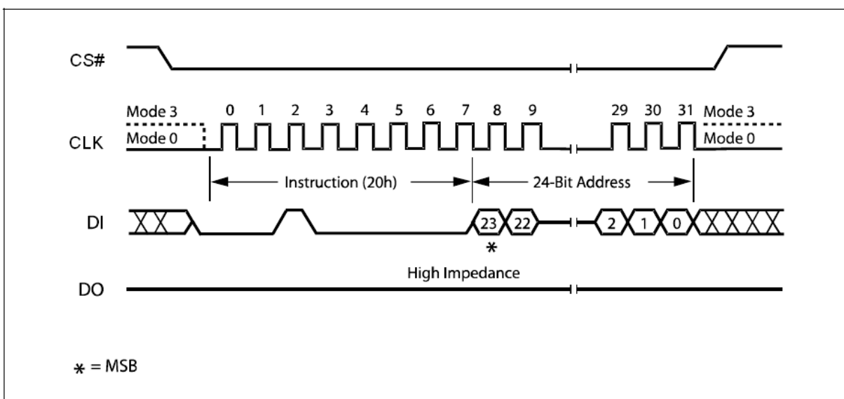
Figure 19. Sector Erase Instruction Sequence Diagram
