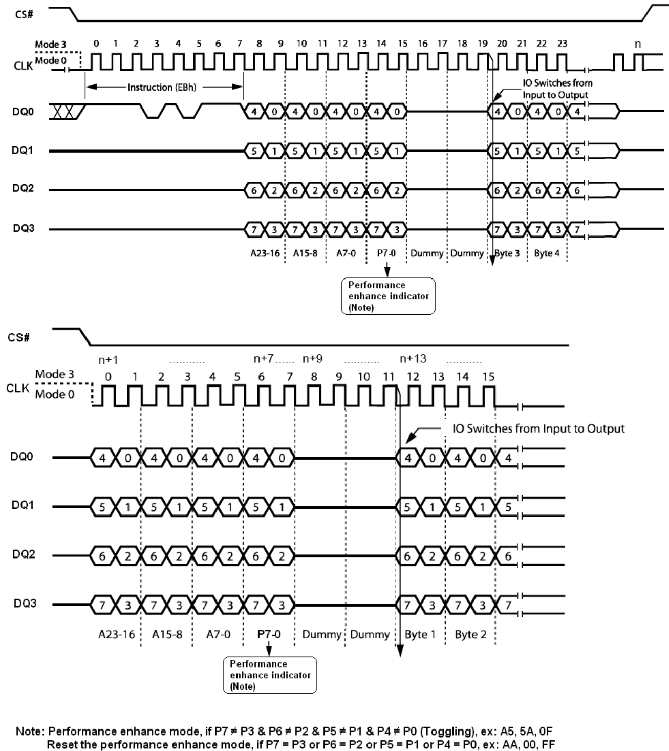
Figure 17. Quad Input/Output Fast Read Enhance Performance Mode Sequence Diagram
