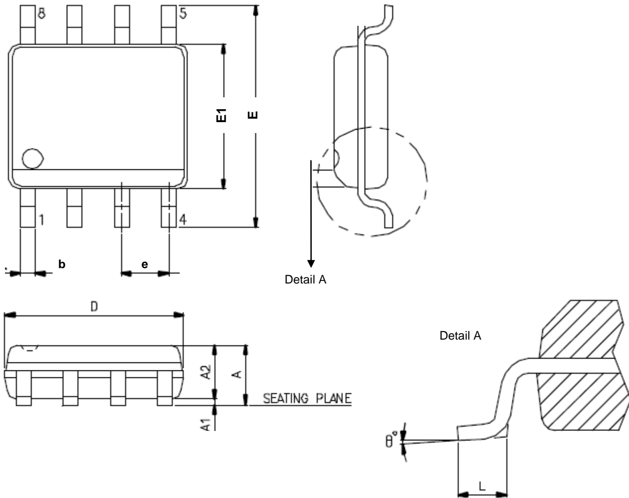
Figure 34. SOP 8 ( 150 mil )
