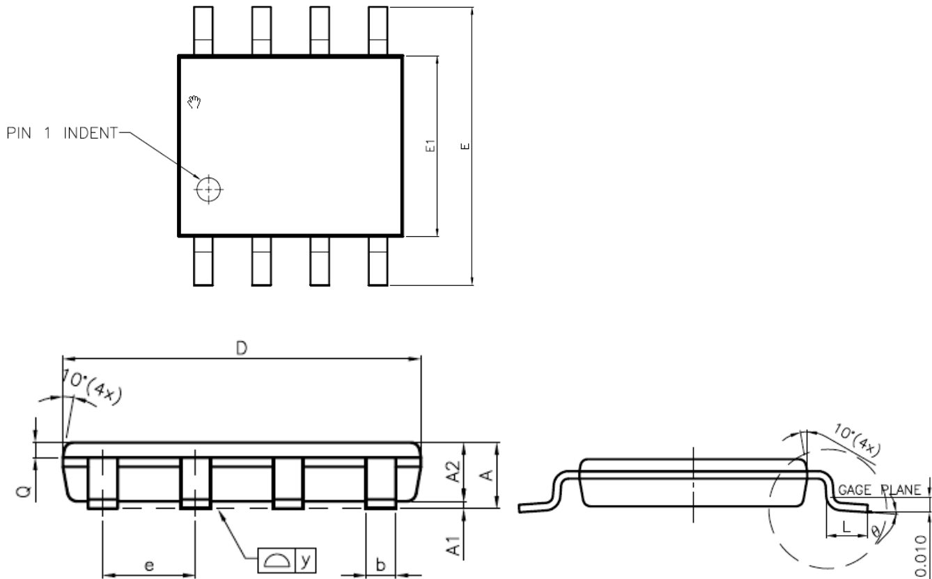
Figure 35. VSOP 8 ( 150 mil )
