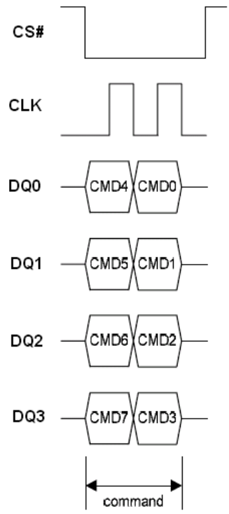
Figure 22.1 Chip Erase Sequence in QPI Mode
