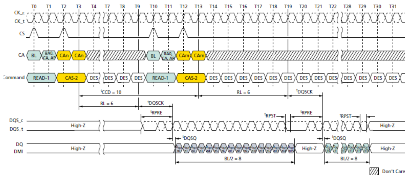
Consecutive READ: t_{\text{CCD}} = \text{MIN} + 2 , Preamble = Toggle, 0.5nCK Postamble
