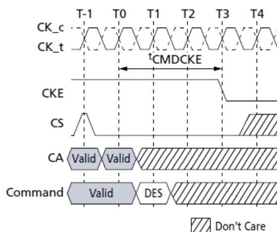
t_{\text{CMDCKE}} Timing
