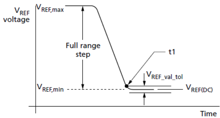
V REF(DQ) Full Step from V REF,max to V REF,min
