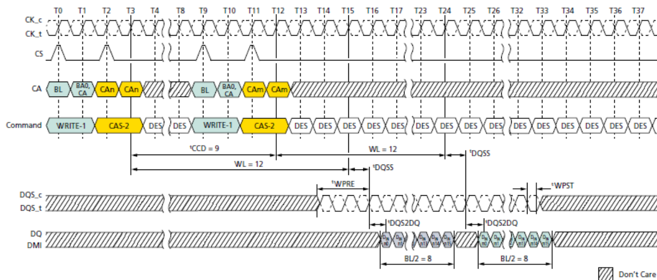
Consecutive WRITE: t'_{CCD} = \text{MIN} + 1 , 0.5nCK Postamble
