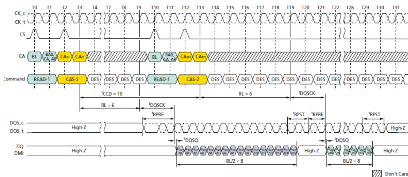
Consecutive READ: t_{\text{CCD}} = \text{MIN} + 2 , Preamble = Toggle, 1.5nCK Postamble
