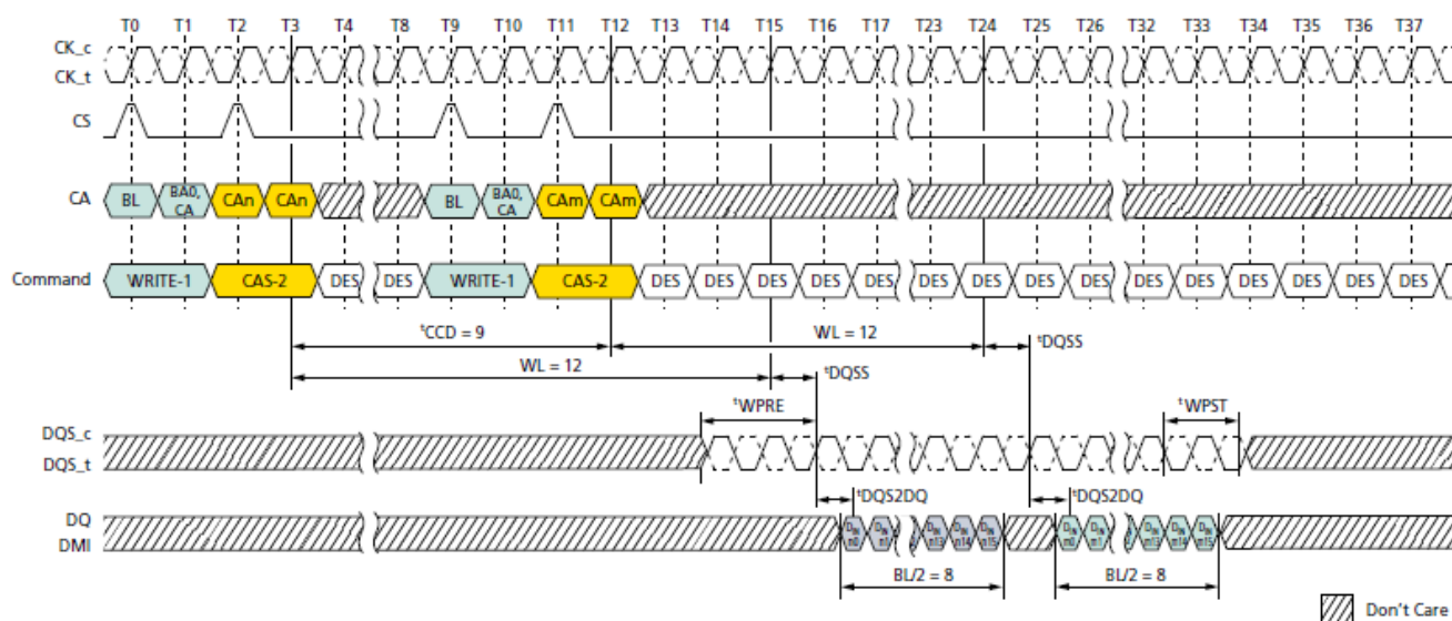
Consecutive WRITE: t'_{CCD} = \text{MIN} + 1 , 1.5nCK Postamble
